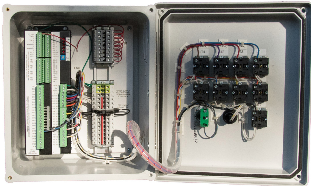
LS-8C LEAK SENTRY
